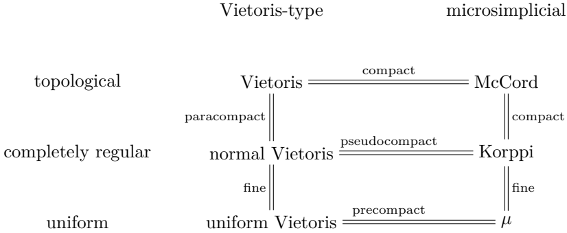
FIG. 1.1: Double lines indicate isomorphisms. The label of each line indicates the condition for that isomorphism.
