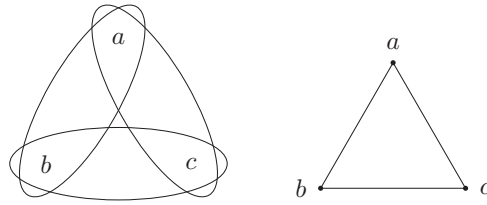
FIG. 2.1: The left depicts the three point space X := \{a, b, c\} equipped with the cover \lambda := \{\{a, b\}, \{a, c\}, \{b, c\}\} . The right depicts a geometric realisation of \mathcal{V}(X, \lambda, \in) within the plane.
