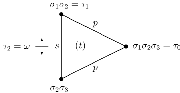
Figure 3. The polarity \omega acting on \Gamma(\mathcal{P}) .
