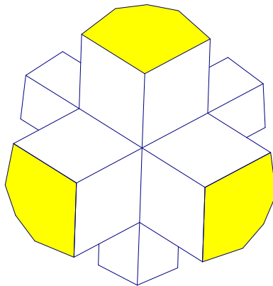
Figure 2. A chiral map of type \{4, 6|6\}
