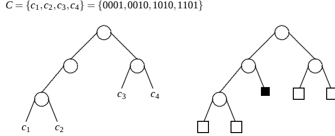
Fig. 2: An example for a set of code words (keys) C , the resulting trie and the corresponding generalized extended binary tree.
