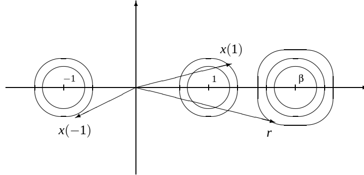
Fig. 2: Two possible noisy bits x(1) and x(-1) and a noisy reference r in the case N = 1 .
