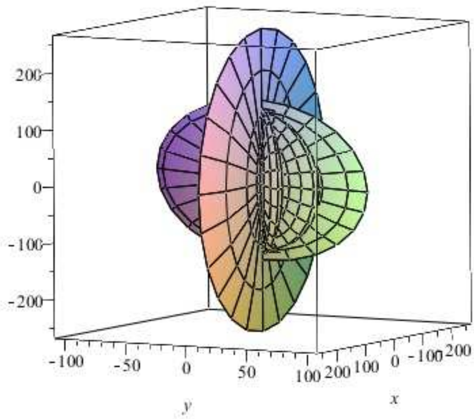
The regularized solution (eps=1e-003)
