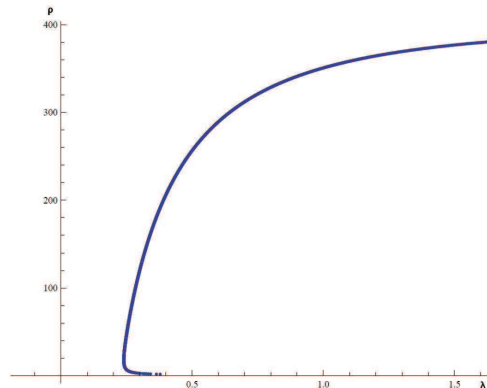
Figure 9: \lambda vs \rho when a = 100, b = \frac{1}{4} and c = 74 - (2 solutions)
