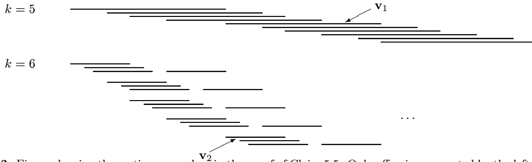
FIGURE 2. Figure showing the vertices \mathbf{v}_1 and \mathbf{v}_2 in the proof of Claim 5.5. Only offspring generated by the left neighbors of \mathbf{v}_1 are shown.
