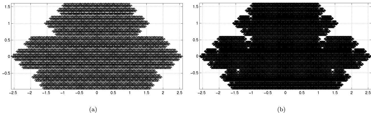
FIGURE 3. (a) The attractor F in Example 5.6. (b) The attractor F in Example 5.7.
