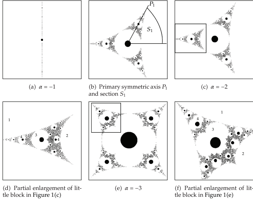
Figure 1: General M-sets and their periodic region.
