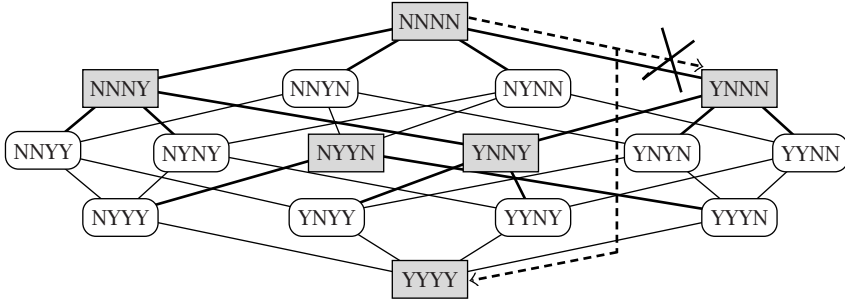
FIGURE 3.1. The hypercube Q_4 has an asymmetric cover consisting of 6 asymmetric balls of radius 1, centered at the gray rectangular vertices; children of ball centers are connected upward to their respective parents by bold lines. In relaxing to a cover by 1-sets, the child of NNNN obtained from changing the first “N” to “Y” can be taken as YYYY instead of YNNN, yielding an optimal 1-set cover of size 5.
