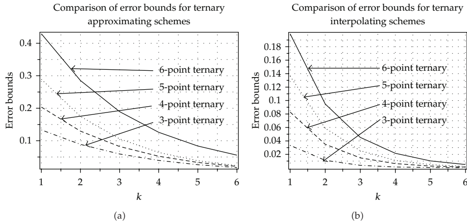
Figure 1: Comparison: error bounds between k th level control polygon and limit curves of different subdivision schemes.
