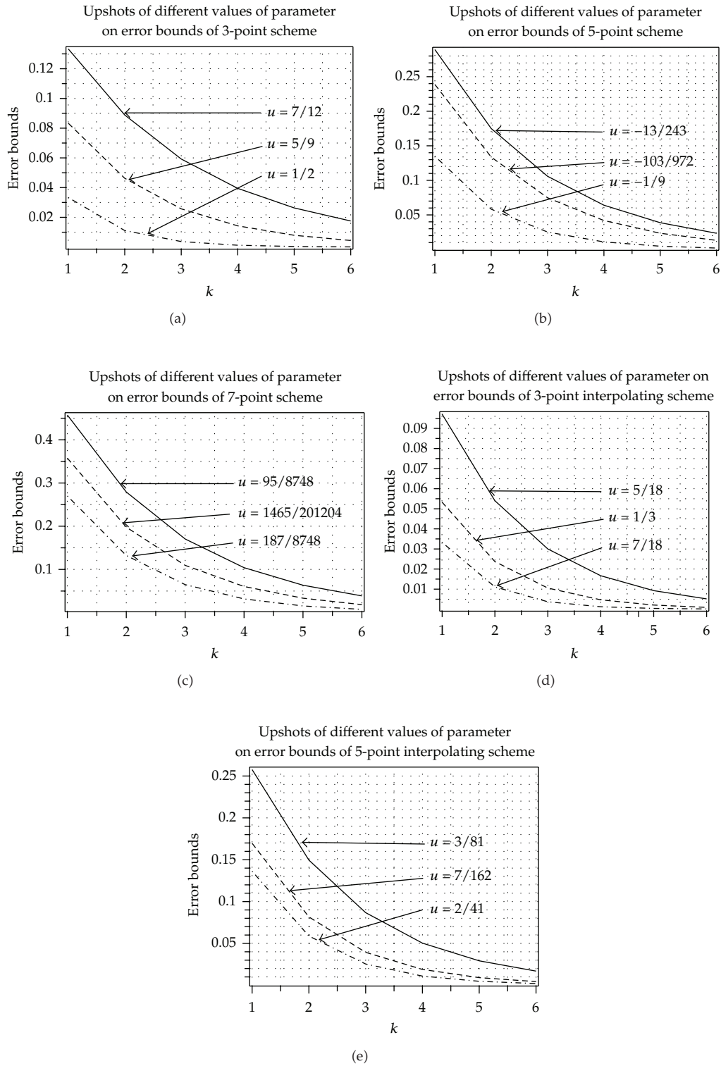
Figure 3: Comparison: error bounds between k th level control polygon and limit curves generated by approximating and interpolating schemes (3.11)–(3.16), respectively.
