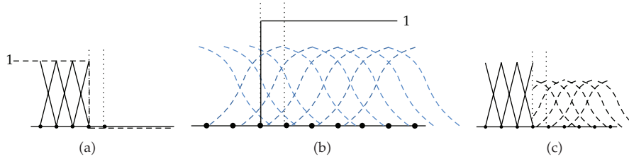
Figure 2: Combination of shape functions in an interfacial area of FEM and FMLS RKM. (a) Shape functions of FEM, (b) shape functions of FMLS RKM, and (c) shape functions of hybrid method. Shape function of FMLS RKM is fully adopted as shape function of the interfacial area (inside two vertical dotted lines).
