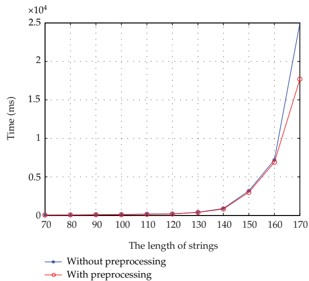
Figure 6: Performance of FACC with/without preprocessing on 20 amino acid sequences ( |\Sigma| = 20 ) with lengths from 70 to 170.
