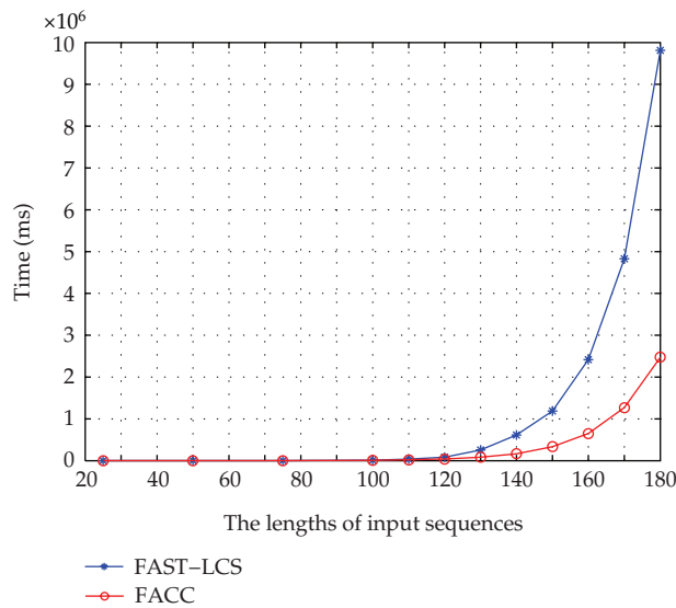
Figure 4: The time performance comparison between FACC and FAST-LCS on 20 DNA sequences ( |\Sigma| = 4 ) with lengths from 25 to 180.
