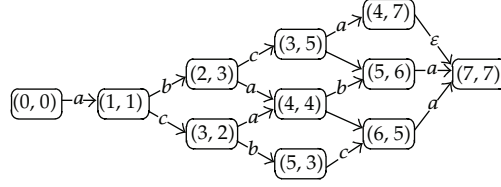
Figure 3: The common subsequence Atm of the sequences S'_1 and S'_2 .
