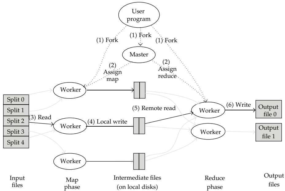
Figure 1: The execution framework of MapReduce.
