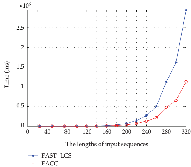
Figure 5: The time performance comparison between FACC and FAST-LCS on 20 amino acid sequences ( |\Sigma| = 20 ) with lengths from 25 to 320.
