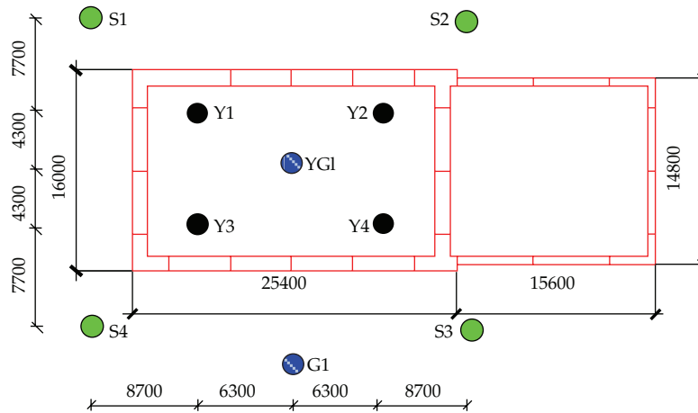
Figure 5: Dewatering wells distributed around southern airshaft excavation (unit: mm).
