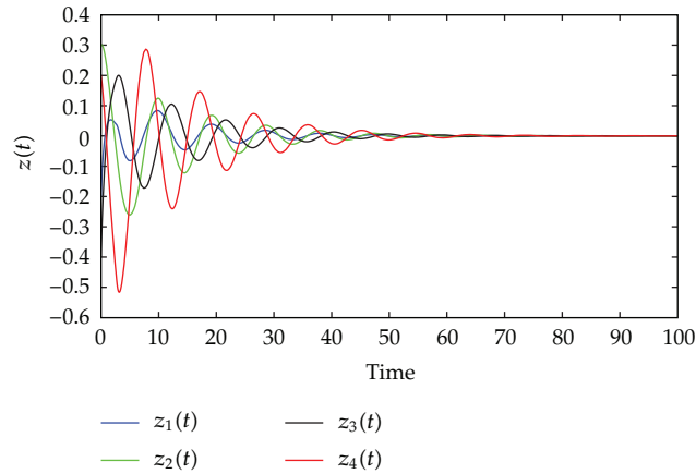
Figure 1: The dynamical behavior of z(t) .
