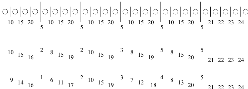
Figure 7. Face representation and extension.
