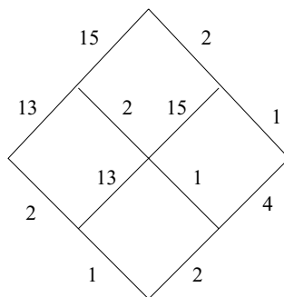
Figure 3. Revised chain-labelling which incorporates block sort.
