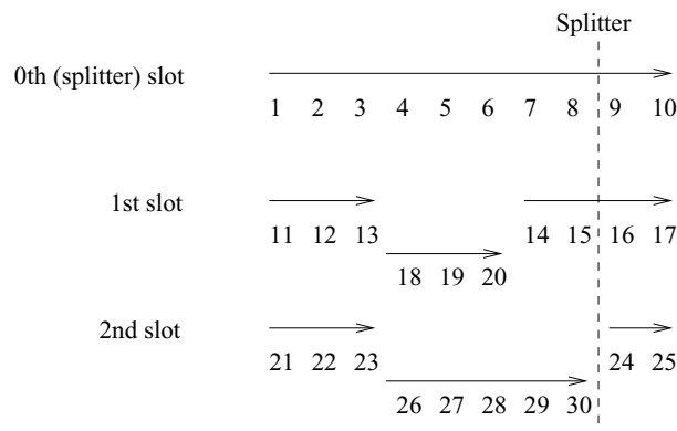
Figure 6. Facet with minimal face of support 8, 17, 28.
