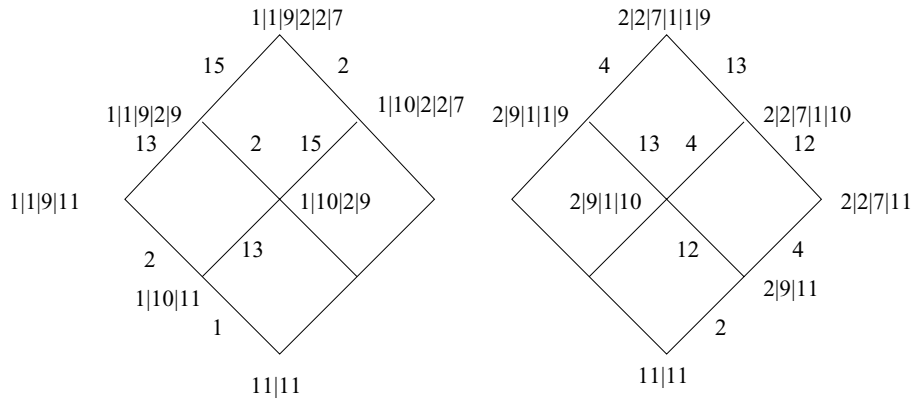
Figure 2. First approximation at a chain-labelling.
