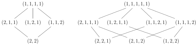
Fig. 2 Thin compositions under refinement
