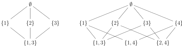
Fig. 1 Sparse subsets under \preceq
