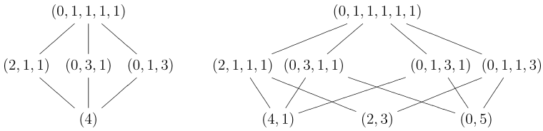
Fig. 3 Almost-odd compositions under refinement
