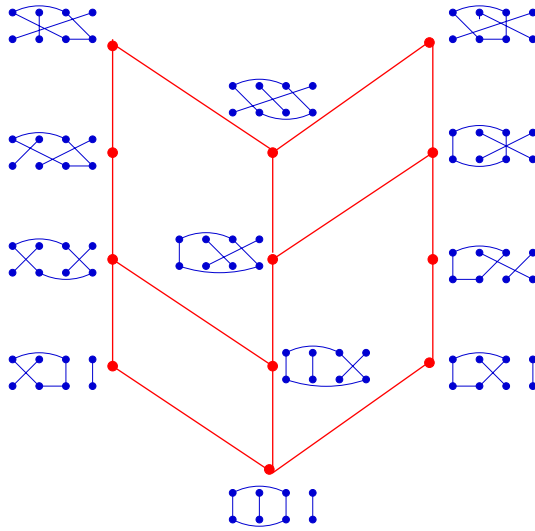
Fig. 6 The component of P_4 corresponding to \mathcal{A} = \{1, 4\}\{2\}\{3\}
