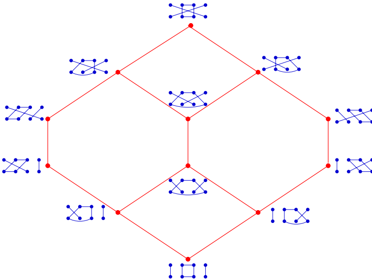
Fig. 5 The component of P_4 corresponding to \mathcal{A} = \{1\}\{2, 3\}\{4\}
