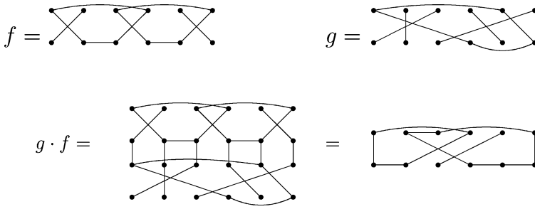
Fig. 2 Product of uniform block permutations
