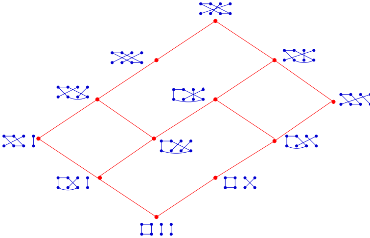
Fig. 4 The component of P_4 corresponding to \mathcal{A} = \{1, 2\}\{3\}\{4\}
