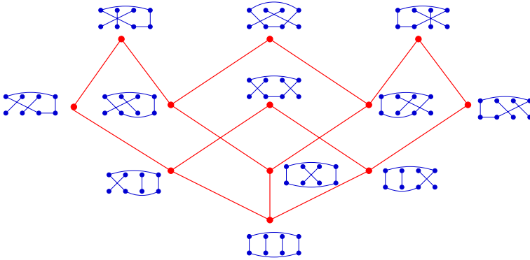
Fig. 6 The component of P_4 corresponding to \mathcal{A} = \{1, 4\}\{2\}\{3\}
