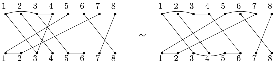
Fig. 1 Two graphs representing the same uniform block permutation
