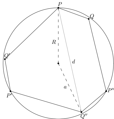
Figure 5.2: Obtaining the extremal sets
