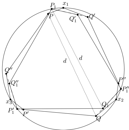
Figure 5.1: Reduction to 3-rotationally symmetric hexagons
