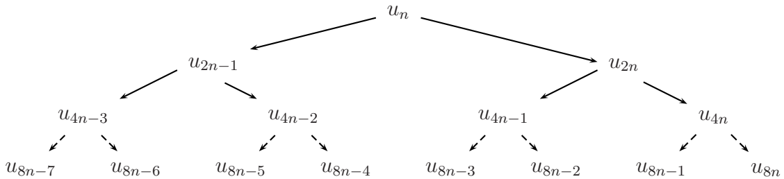
Figure 4: The extended tree for u_n with L = 3 and a = 2 .
