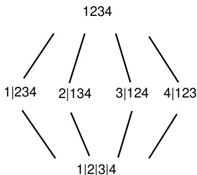
Figure 1: The Hasse Diagram for \Pi_4^{\text{odd}}
