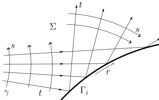
Figure 4: Parametrization of \Sigma by s and t .
