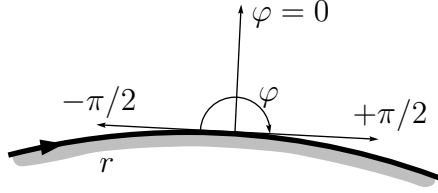
Figure 3: Orientation of r and \varphi .
