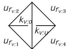
Figure 6: Tetrahedron around a vertex
