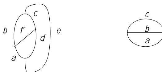
Figure 1: Tet and theta
