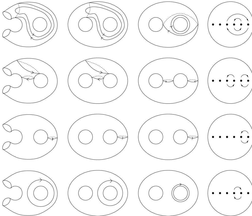
Figure 3: The four maps [TT_a]; [TT_b]; [T_m] , and [T_l] , and their images in M(\Sigma_2) and M(S^2; 6)
