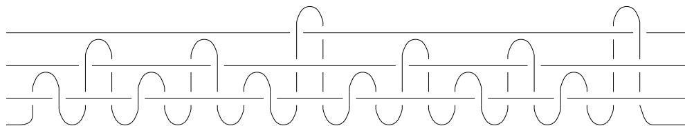
Figure 1: A Brunnian sphere braid with four strands
