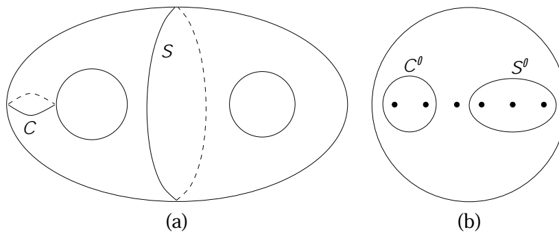
Figure 2: (a) Example of S and C (b) Example of S^\theta and C^\theta
