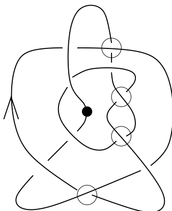
Figure 4: The knot 10_{152} We have indicated, once again, the crossings needed to unknot 10_{152} , and also the distinguished edge ( \epsilon_0 , with the dark circle) used in the decorated knot projection for the proof of Proposition 4.3.
