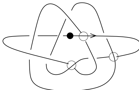
Figure 5: Local filtration level contributions A decorated knot projection for 10_{161} , showing that it has unknotting number at least 3.
