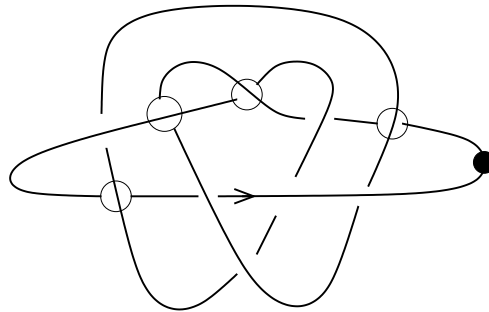
Figure 3: The knot 10_{139} We have circled four crossings: when these are switched, the new knot is the unknot. The black dot indicates the distinguished edge ( \epsilon_0 ) used in the decorated knot projection.
