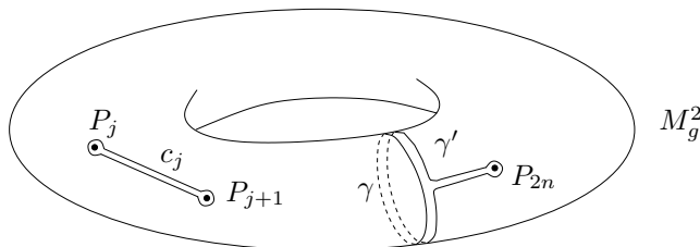
Figure 4: The points P_j, P_{j+1} , and P_{2n} of the underlying surface M correspond to singularities of \psi of odd degree. The paths \gamma and \gamma' are homologous in H_1(M; \mathbb{Z}_2) , but holonomy along \gamma and along \gamma' is different. Holonomy along the path c_j is obviously trivial.
