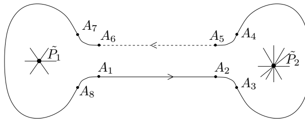
Figure 5: A path \tilde{c}_j on the covering surface obtained by lifting the path \tilde{c}_j . Since \tilde{P}_j, \tilde{P}_{j+1} \in \tilde{M} are ramification points, the segments A_1A_2 and A_6A_5 are located on “different sheets” of the covering \tilde{M} \rightarrow M , and are not near to one another.
