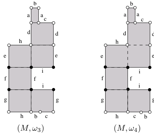
Figure 3: Two points (M, \omega_3) and (M, \omega_4) in the stratum \mathcal{H}(2, 4)
