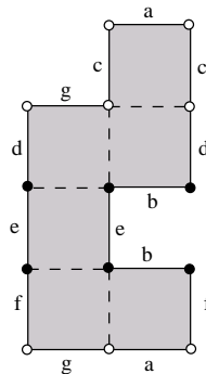
Figure 1: A point in the stratum \mathcal{H}(2, 2)
