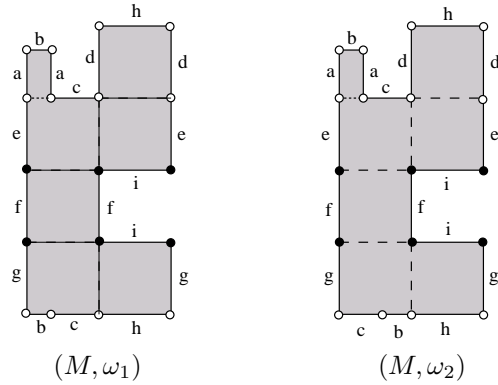
Figure 2: Two points (M, \omega_1) and (M, \omega_2) in the stratum \mathcal{H}(2, 4)
