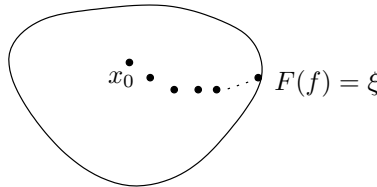
Figure 11: Wolff–Denjoy result: orbit of f
