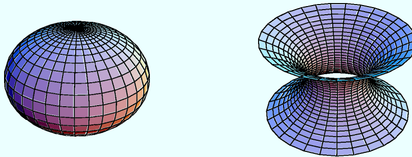
Figure 1. Sphere and its dual surface (the catenoid) on the right side
