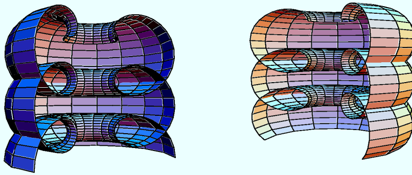
Figure 3. Slices of the immersions of the nodoid and its dual surface on the right side for k = 0.555556
