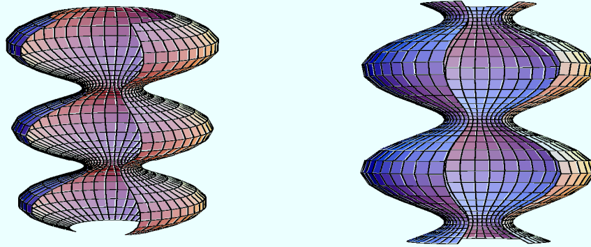
Figure 2. Some open parts of the unduloid and its dual surface on the right side for k = 0.555556
