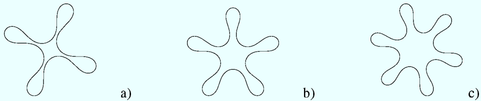
Figure 6. Closed non self-intersecting curves obtained by the solution (23) and corresponding to: a) \mu = 0.477 , \sigma = 1 ; b) \mu = 0.347 , \sigma = 1 and c) \mu = 0.269 , \sigma = 1 .
