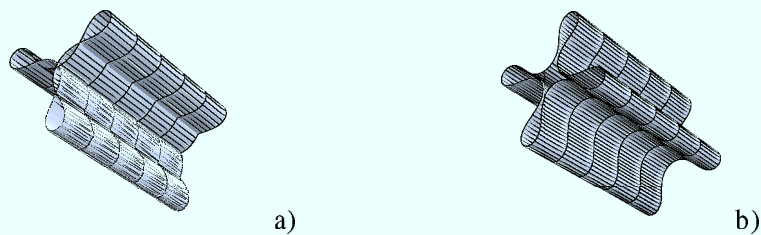
Figure 8. Surfaces generated by the directrices shown in: a) Fig. 5b); b) Fig. 6a).
