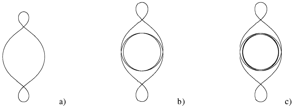
Figure 2. Closed self-intersecting two-fold symmetry curves obtained by the solution (18) and corresponding to: a) \mu = 0.238 , \sigma = 0.042 ; b) \mu = 0.199 , \sigma = 0.034 ; c) \mu = 0.193 , \sigma = 0.033 .
