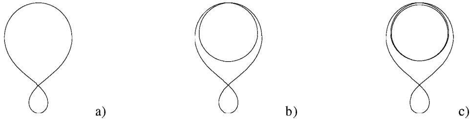
Figure 1. Closed self-intersecting one-fold symmetry curves obtained by the solution (18) and corresponding to: a) \mu = 0.208 , \sigma = 0.036 ; b) \mu = 0.195 , \sigma = 0.033 ; c) \mu = 0.192 , \sigma = 0.032 .
