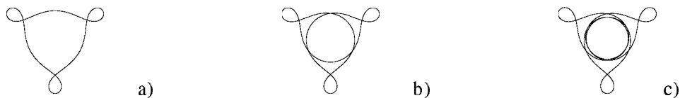
Figure 3. Closed self-intersecting curves with three-fold symmetry obtained by the solution (18) and corresponding to: a) \mu = 0.268 , \sigma = 0.047 ; b) \mu = 0.223 , \sigma = 0.039 and c) \mu = 0.202 , \sigma = 0.035 .
