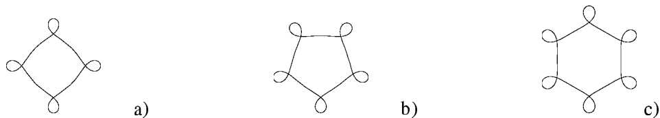
Figure 4. Other closed self-intersecting curves obtained by the solution (18) and corresponding to: a) \mu = 0.299 , \sigma = 0.052 ; b) \mu = 0.330 , \sigma = 0.057 ; c) \mu = 0.361 , \sigma = 0.061 .
