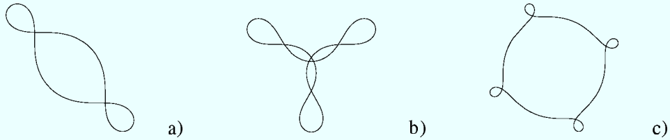
Figure 5. Closed self-intersecting curves generated by the solution (23) and corresponding to the set of parameters: a) \mu = 1.449 , \sigma = 1 ; b) \mu = 0.732 , \sigma = 1 ; c) \mu = 0.5 , \sigma = 0.046 .
