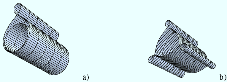
Figure 7. Surfaces generated by the directrices shown in: a) Fig. 1b); b) Fig. 3a).
